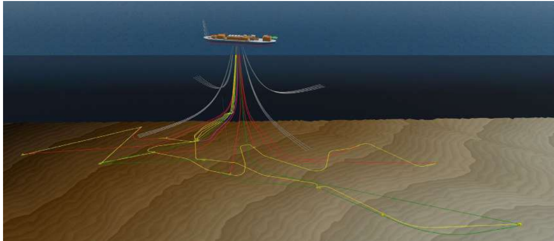
Figure 4.3 Pecan Phase 1a and 1b illustration
