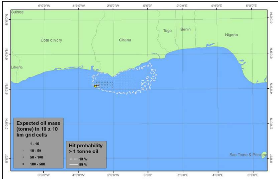
Figure 6.10 Annual Surface Oiling Probabilities for Scenario 2
