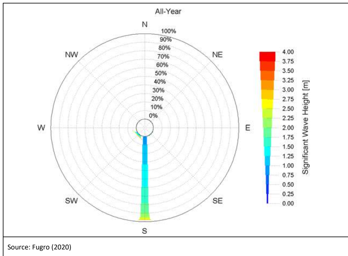
Figure 5.8 Mean Wave Direction in the Project Area (All-Year)
