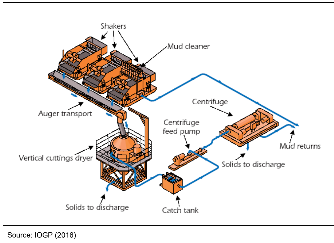
Figure 4.12 Advanced Solid Control System Including a Secondary Treatment
