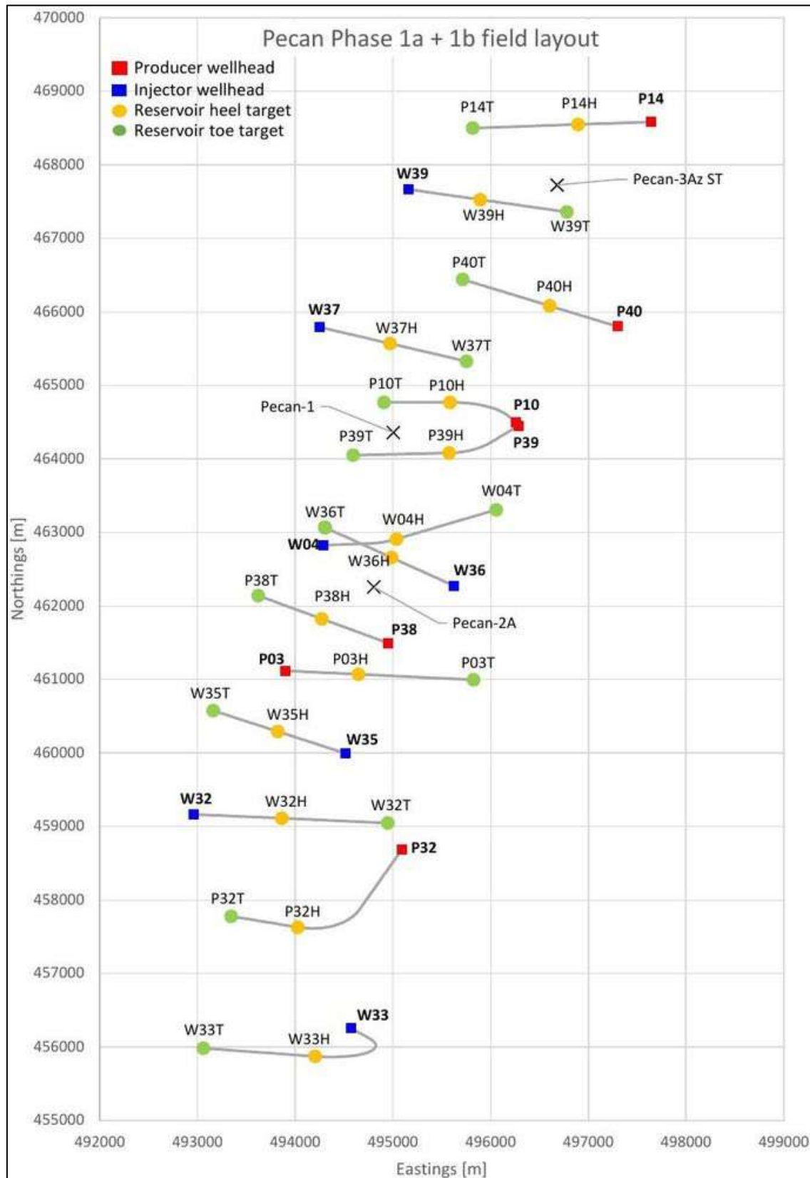
Figure 4.2 Pecan Phase 1 Field Layout / Wellbore trajectories
