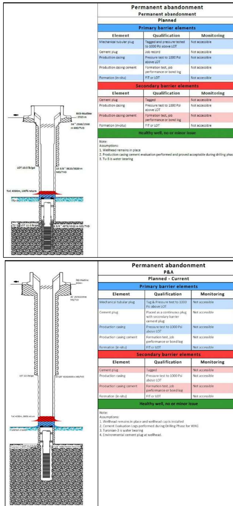
Figure 9.1 Permanent Abandonment for Producer (top) and Injection (bottom) Wells
