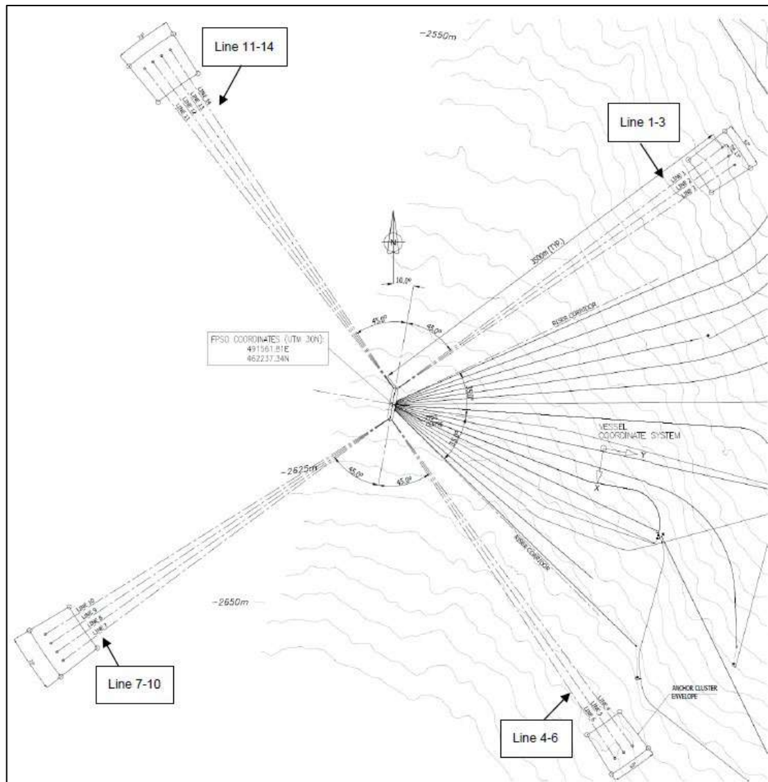
Figure 4.7 FPSO Mooring Spread
