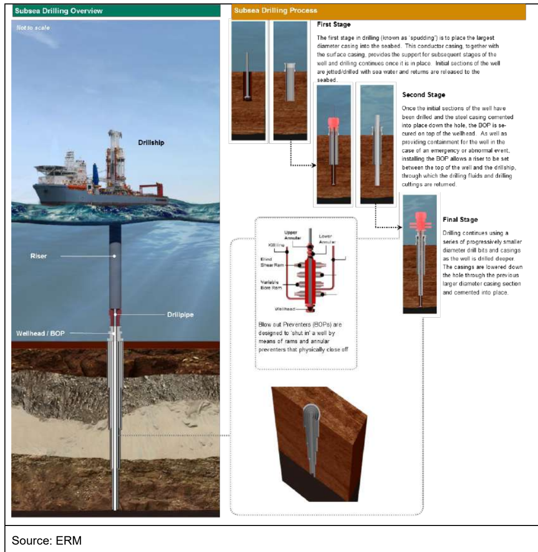
Figure 4.9 Typical Drilling Operations using a Drill Ship
