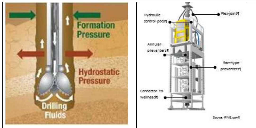
Figure 4.8 Hydrostatic Pressure and BOP Schematic
