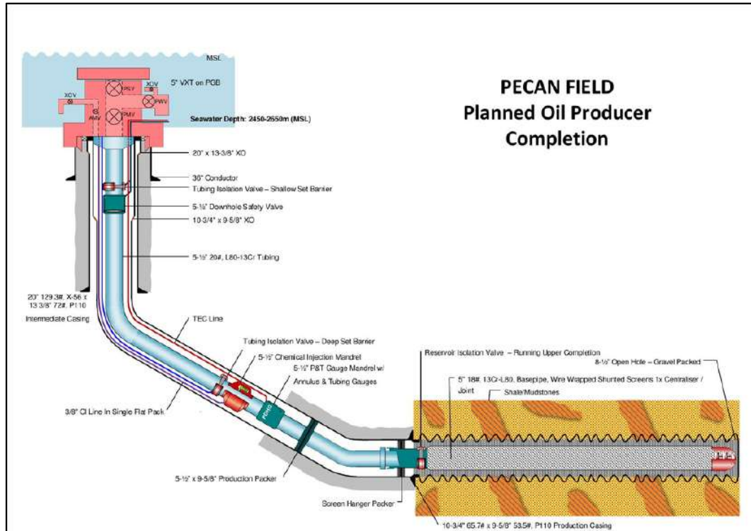
Figure 4.13 Oil Producer Completion
