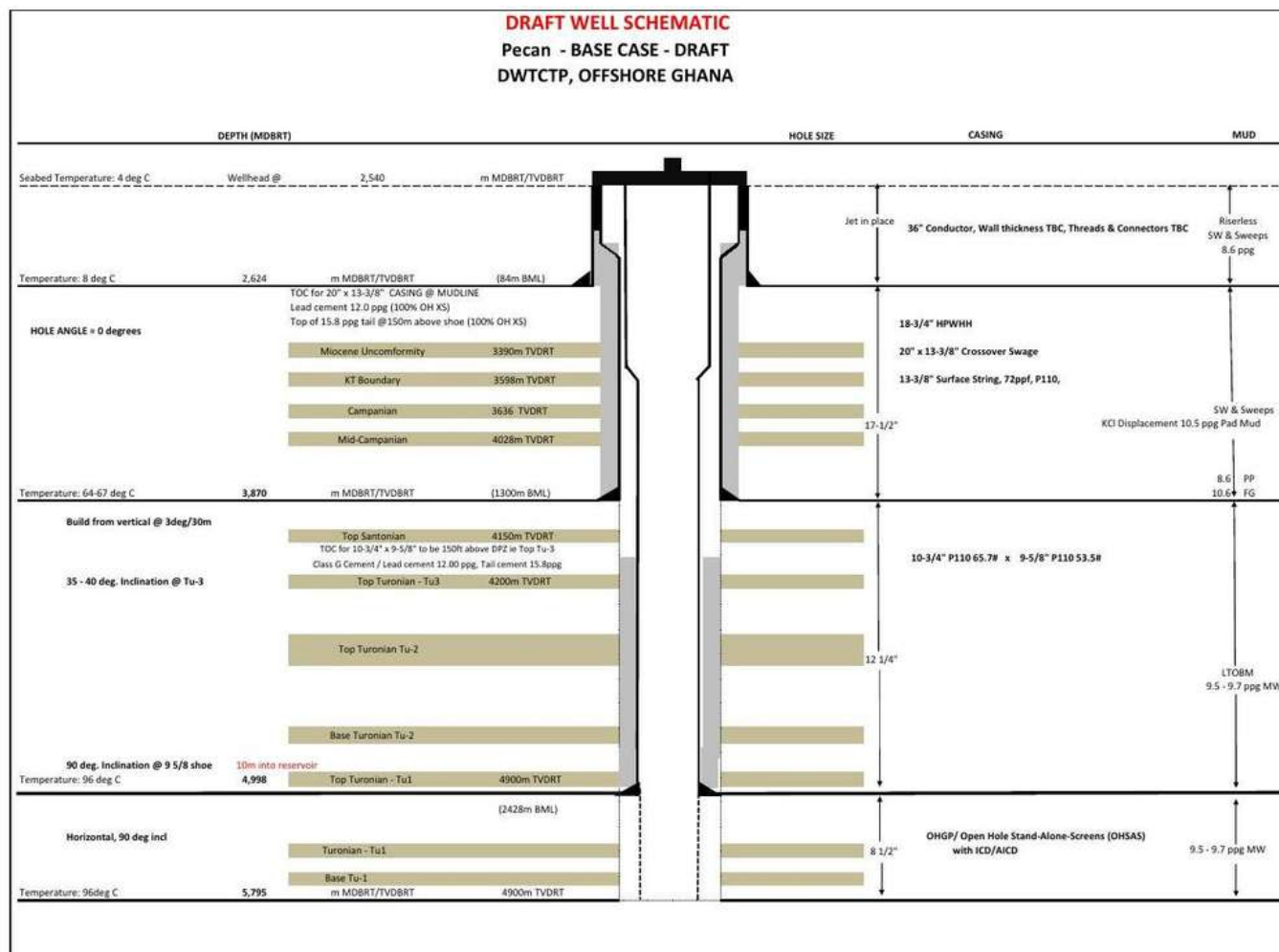
Figure 4.11 Well Bore Schematic
