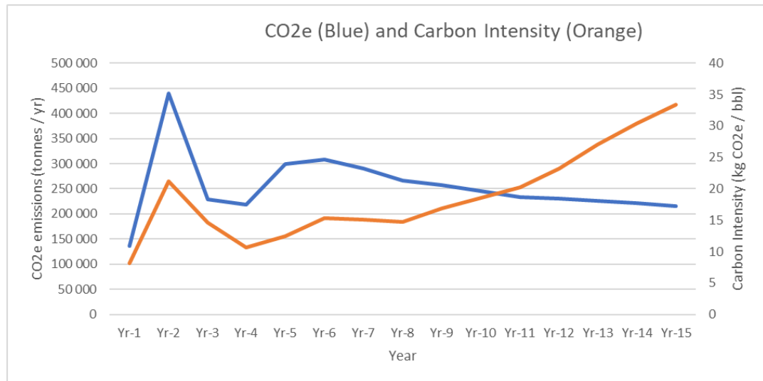
Figure 6.5 Calculated CO2e Emissions and Carbon Intensity for FPSO Operations for 15 years of Production
