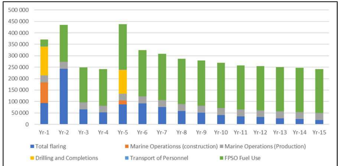
Figure 6.4 Calculated CO 2e Emissions From the Main Project Sources for 15 Years of Production
