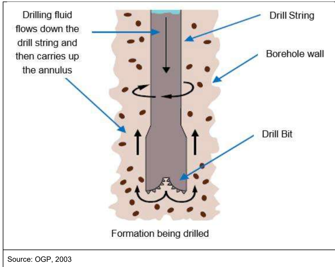
Figure 4.10 Circulation of Drilling Fluid during Drilling
