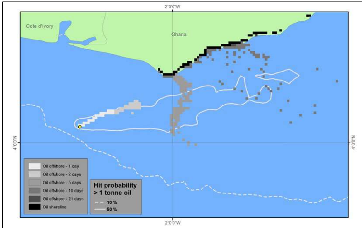
Figure 6.13 Trajectory of Oil Spill Over Time for Simulation with Largest Mass of Oil Reaching the Coast for Scenario 3
