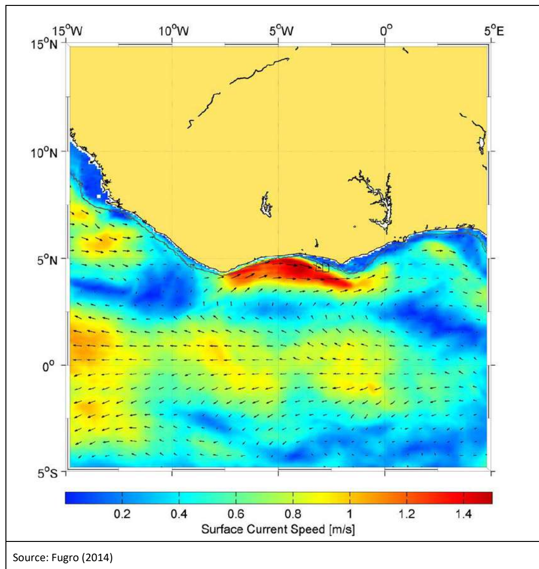
Figure 5.4 Surface Current Speed in the Guinea Current
