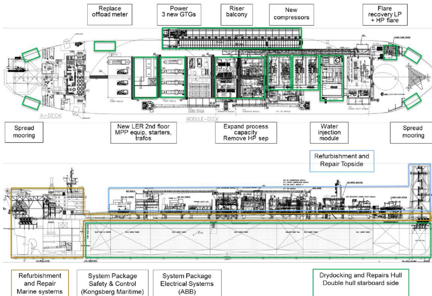
Figure 4.6 Plan View Showing Planned Modifications to FPSO Dhirubhai-1
